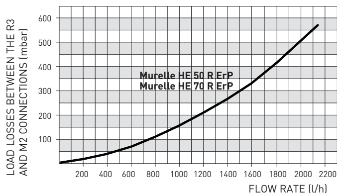
CURVE LOAD LOSSES/CAPACITY BETWEEN THE CONEXIONES R3 and M2
